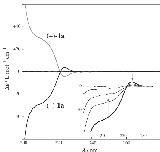
Figure 2. CD spectra of (+)- and (–)- 1a in hexane. Inset spectra are changes during the racemization of (–)- 1a upon heating for 0, 70, 300, 600, and 1080 min at 69 °C.
