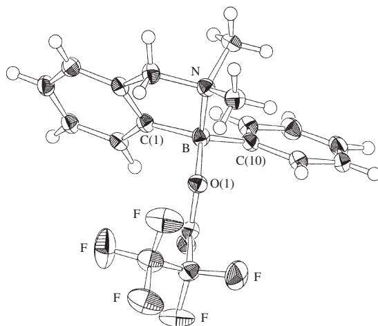
Figure 1. ORTEP diagram of rac - 1a with thermal ellipsoids at 50% probability. B–N 1.668(4) Å, C(1)–B–O(1) 110.4(2), C(10)–B–O(1) 111.8(2), C(1)–B–C(10) 120.2(2)°.
